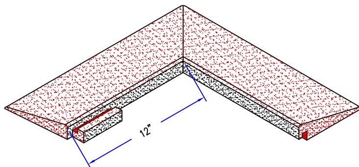
Outside Corner
